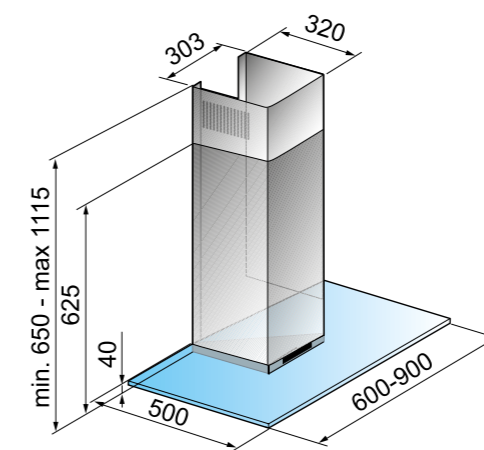
KHC 9971 X KHC 6971 X
