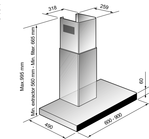
KHC 9770 X KHC 6770 X
