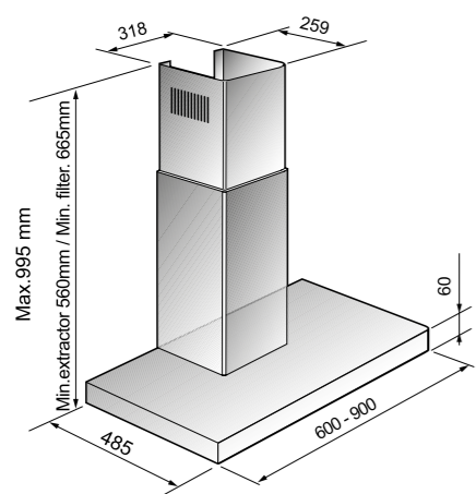
KHC 9957 X KHC 6957 X
