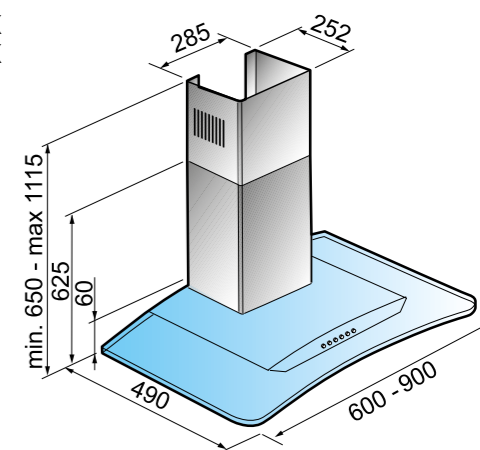
KHC 9954 X KHC 6954 X
