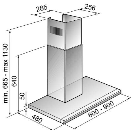
KHC 9973 X KHC 6973 X
