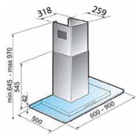
KHC 9956 X KHC 6956 X
